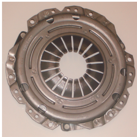
Traditional type Clutch Cover Assembly
