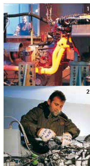
1 | Service life test – test bench
