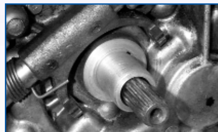
Mainshaft bearing wear (Movement)
