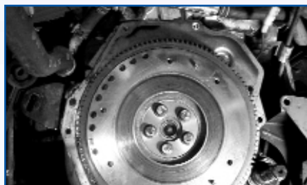
Flywheel wear
