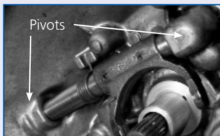
Worn or Seized Release mechanism pivots
