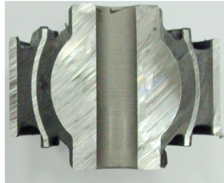
New version (swaged bush)
