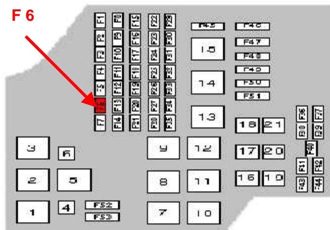
Fuse box engine compartment
