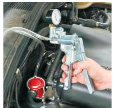
Checking a secondary-air valve with a vacuum hand pump
