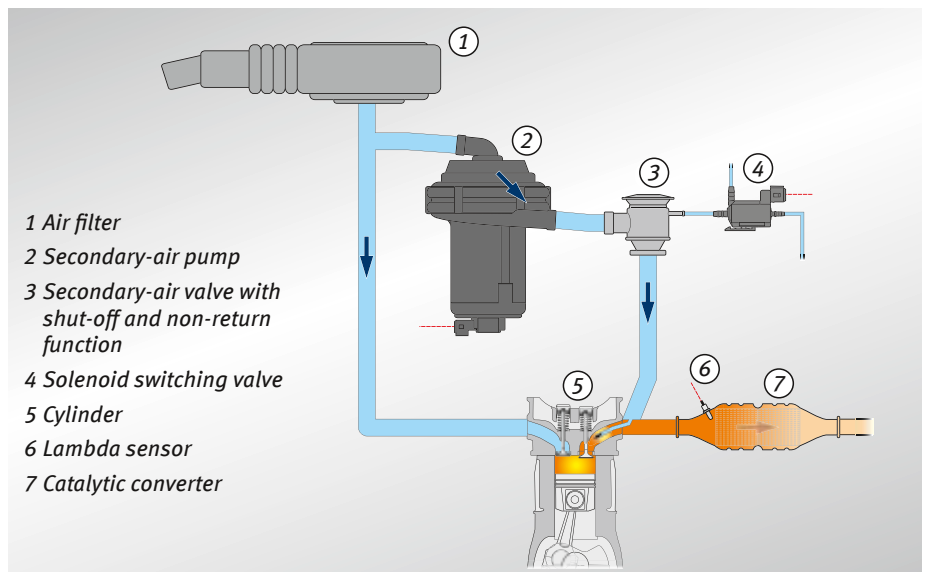
Block diagram of secondary-air system (pneumatically actuated)
