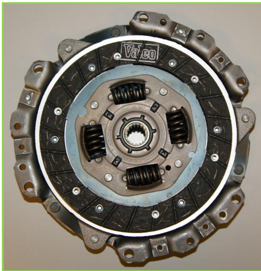
Please note the friction plate is 10mm smaller in diameter than the clutch cover
