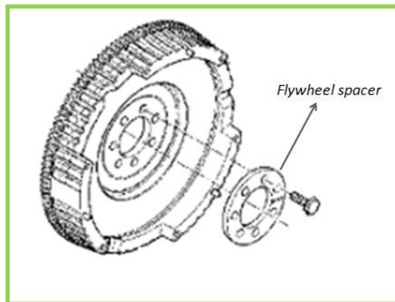
Flywheel, flywheel spacer and bolts
